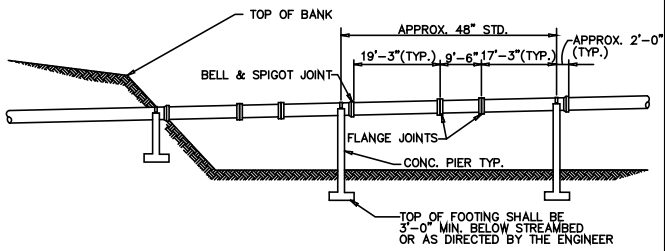
ELEVATED CROSSING – TYPE III (18" AND LARGER PIPE)
