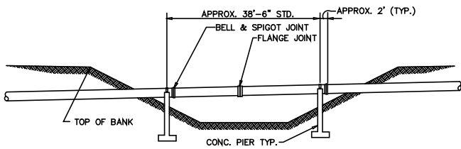
ELEVATED CROSSING – TYPE II
