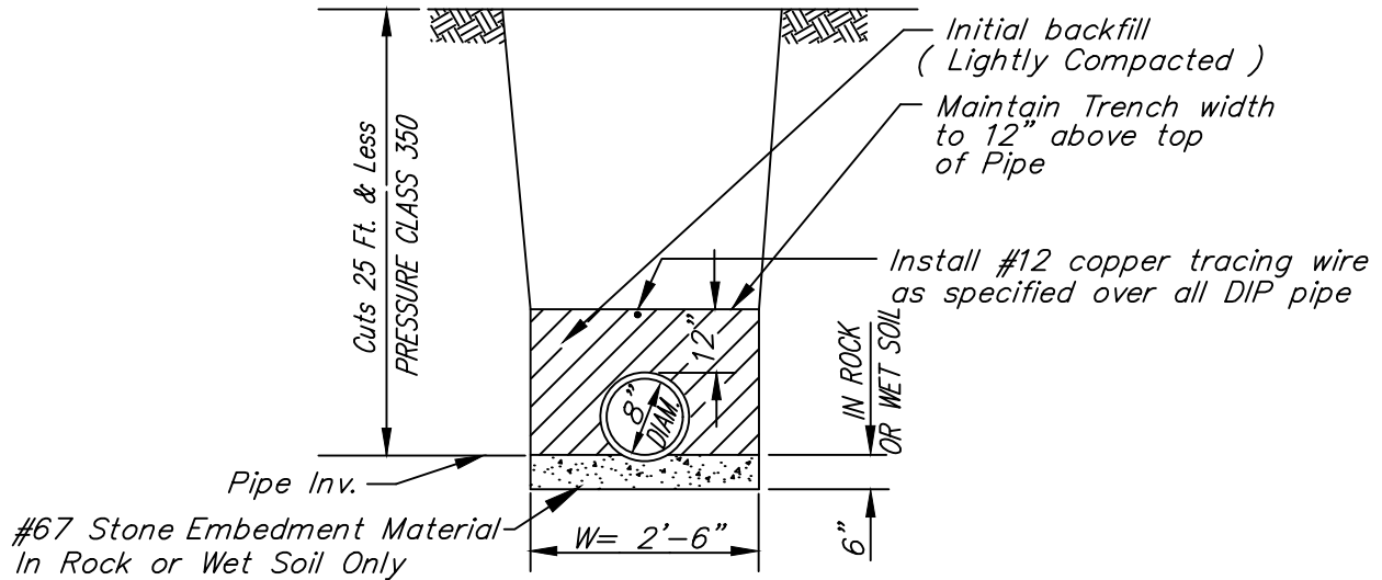
TYPICAL SEWER TRENCH 8" D.I. PIPE CUTS 20 FT. & LESS
