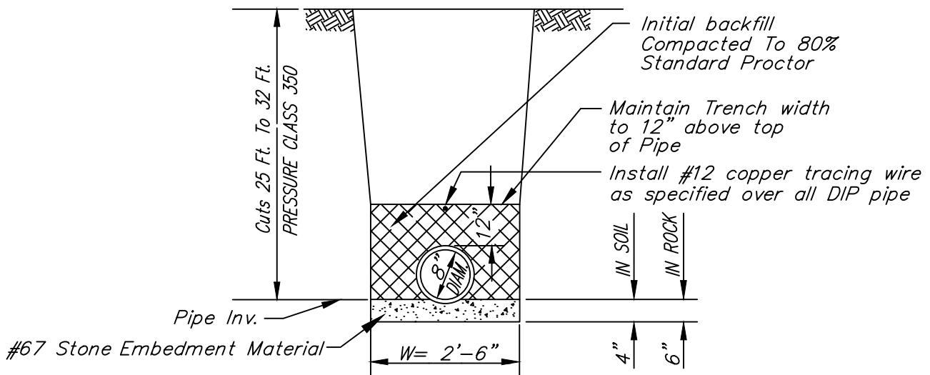
TYPICAL SEWER TRENCH 8" D.I. PIPE CUTS 20 FT. TO 32 FT.
